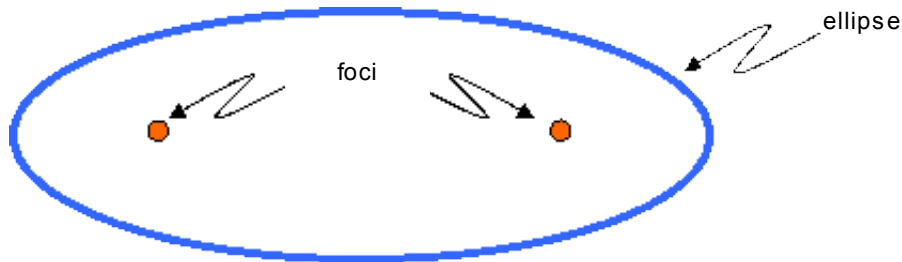
Illustration 1: An ellipse.
